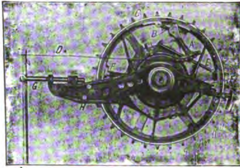
FIG. 469.—The "Duryea" Expanding Break. The two ends of the metal band are separated by the lever, A, and the adjusting screw, B, which is swiveled to the hinge, C. A forward pull on lever, A, through the chain pull, indicated by D, causes the two ends of the band to be thrust apart and bear against the inner surface of the sprocket. The extension spring, E, normally holds the band away from this friction surface. The two lugs, FF, attached to a spider hung on the axis of the sprocket, take the braking effort from the bottom of the band more into the line of travel. A framework, indicated at H and I, supports a leather guard covering both the chain and sprocket.
